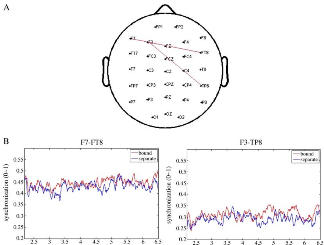
Fig. 3. Greater 6 Hz phase synchronization in the bound than in the separate condition. (A) Phase synchronization significance map for the 6 Hz frequency. Electrode pairs in which the 6 Hz phase synchronization was significantly ( P \leq 0.05 ) different between the bound and separate conditions are plotted on the scalp. Red and blue lines respectively indicate phase synchronization being greater and lesser in the bound than in the separate condition. Here no blue line was obtained. (B) The mean time courses of the 6 Hz phase synchronization of electrode pairs F7-FT8 and F3-TP8.
